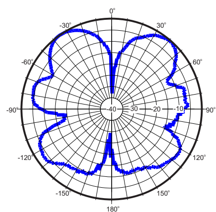
Rad. Pattern E-plane Frequency: 1800 MHz
