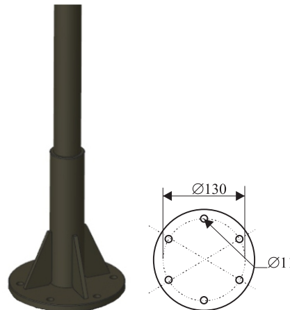
Bolt Pattern for Attachment Type A, B, C
