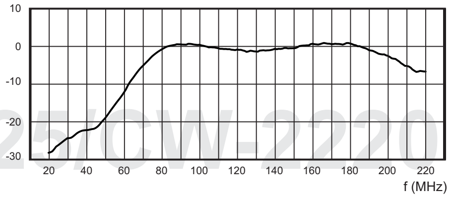
GAIN (dBi)
