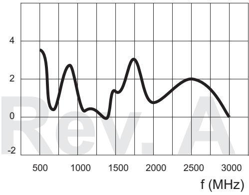
Gain (dBi)
